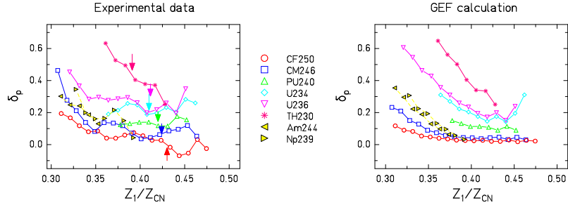
Fig. 2. Local even-odd effect as a function of asymmetry for various fissioning nuclei. The experimental data are shown on the left and the GEF calculation 4 on the right.
