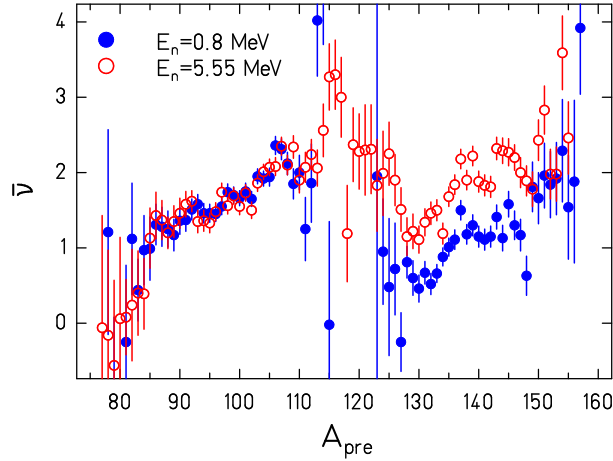
Fig. 1. Average number of prompt neutrons as a function of the primary fragment mass for the neutron-induced fission of ^{237}\text{Np} , data taken from ref. 5
